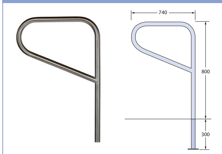
Pennant Stainless Steel Cycle Stands, Crown Point, Denton
