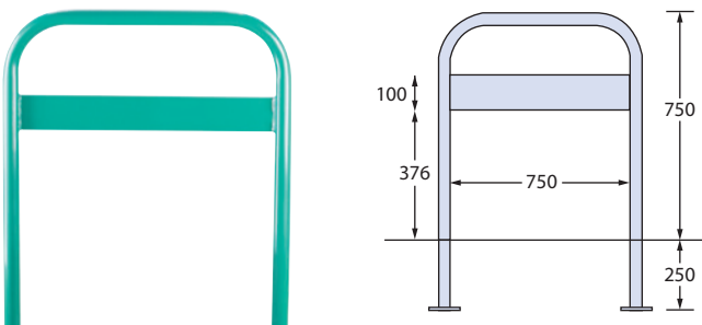
SHEFFIELD CYCLE STAND WITH SIGN BOARD
