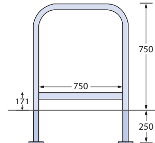
SHEFFIELD CYCLE STAND WITH TAPPING BAR
